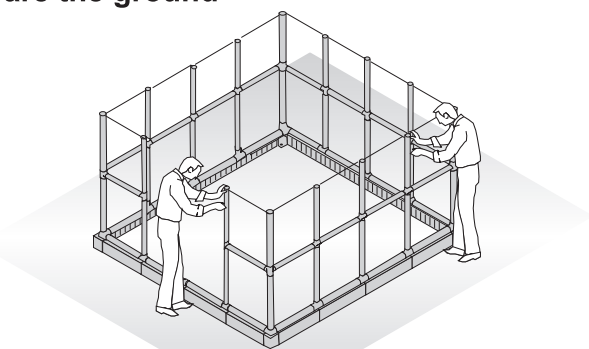
Step III: Build base and walls See From Page 26
