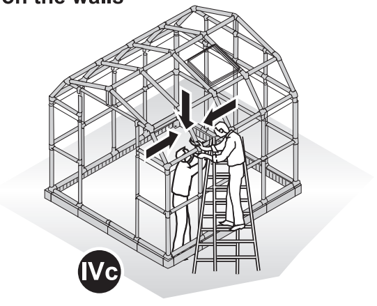
Step IV: Attach the assembled roof on the walls See From Page 33
